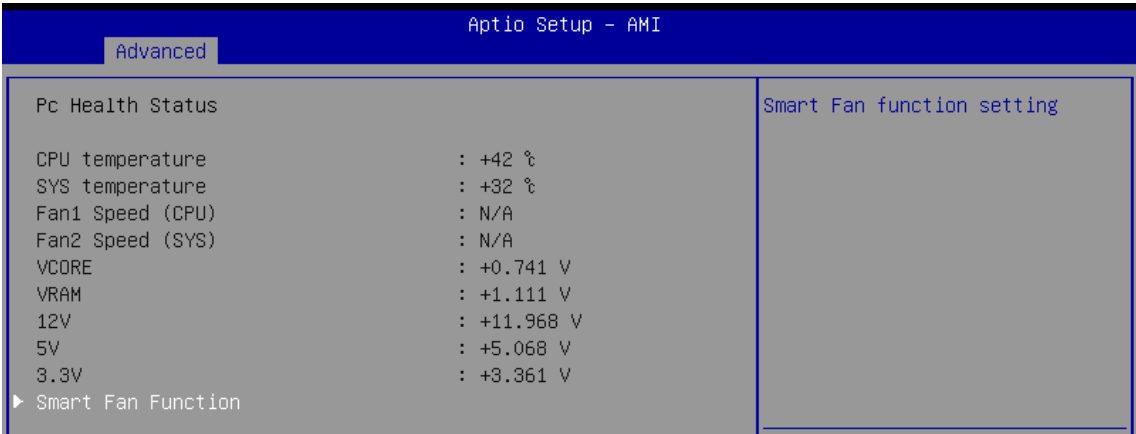
Figure 4-3-7 : Hardware Monitor
