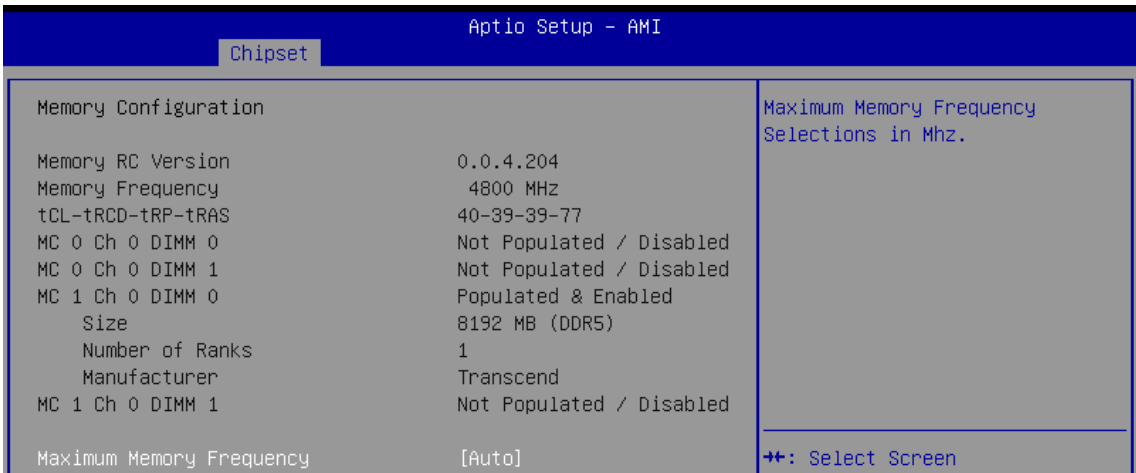
Figure 4-4-2 : Memory Information
