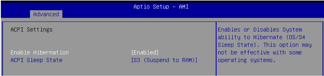
Figure 4-3-5 : ACPI Settings
