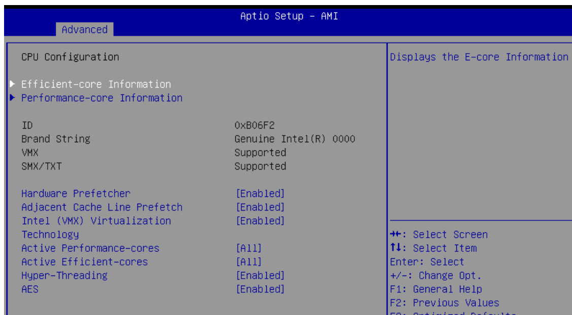
Figure 4-3-1 : CPU Configuration
