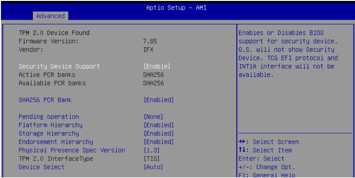
Figure 4-3-4 : Trusted Computing
